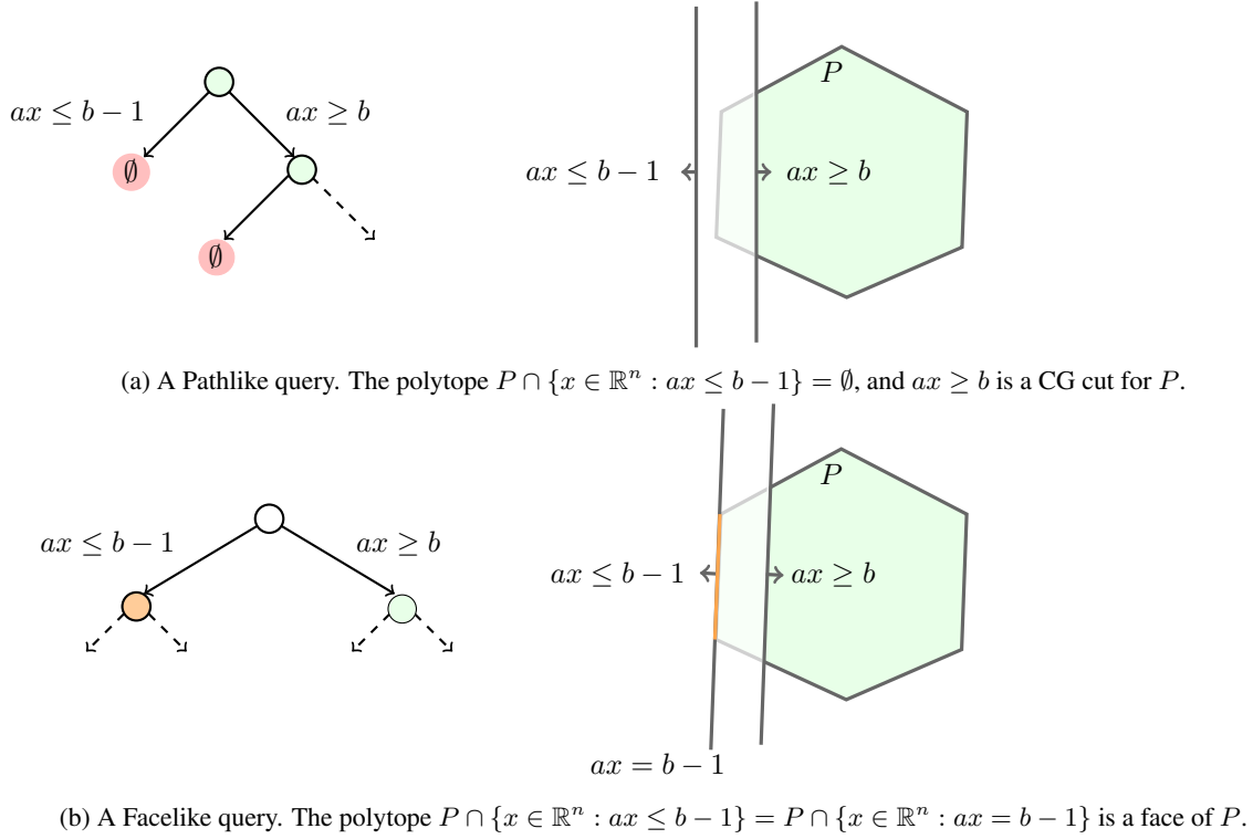
Figure 2: Pathlike and Facelike SP queries on a polytope P . On the left are the proofs and on the right are the corresponding effects on the polytope.
